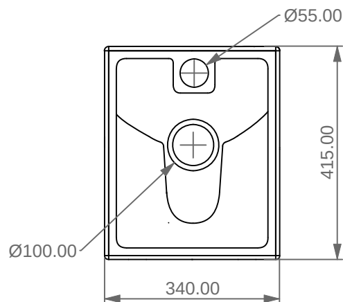
REAR
